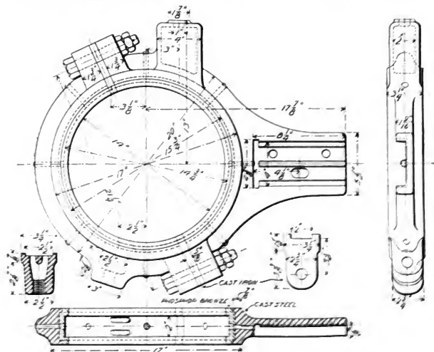
Fig. 1878-1882. Cast Steel Eccentric Strap, Rogers Locomotive Works.
